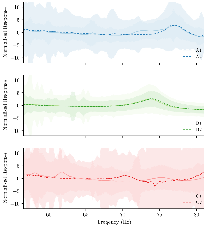
Fig. 7. Feature between 56.56 and 81.56 Hz, for all tailplanes. Shaded region shows one standard deviation around the mean.
