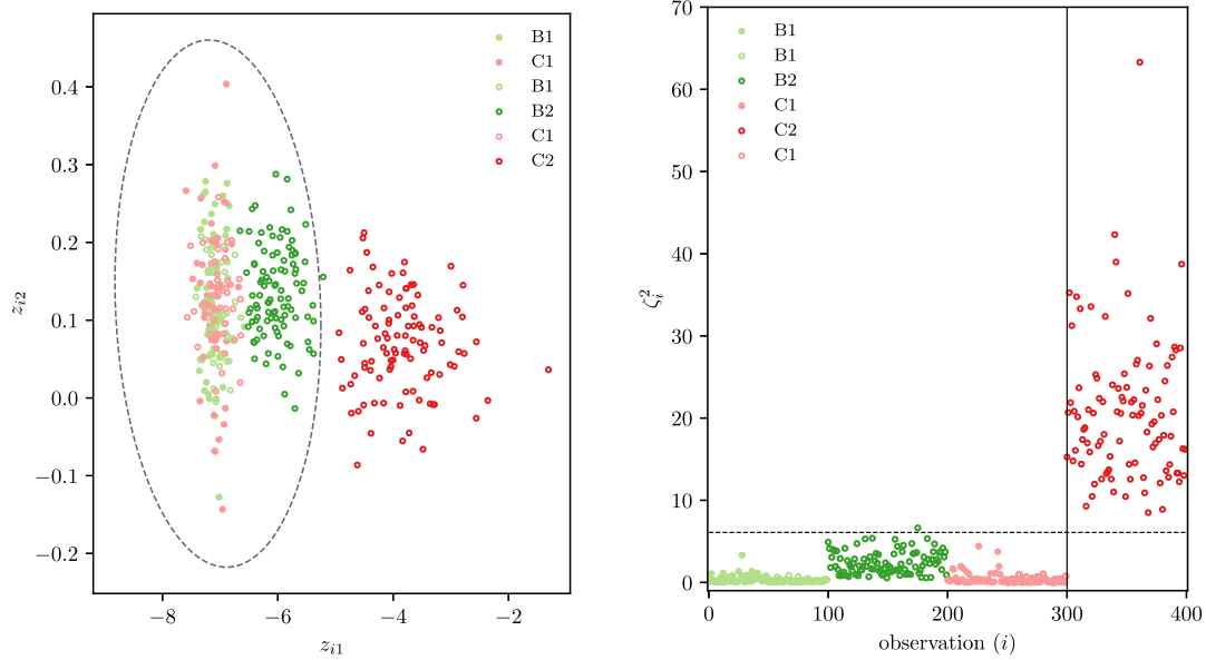
(a) \mathcal{Z} : filled markers \bullet represent training data, hollow markers \circ represent test data. The dashed line shows the confidence ellipse for damage detection.
