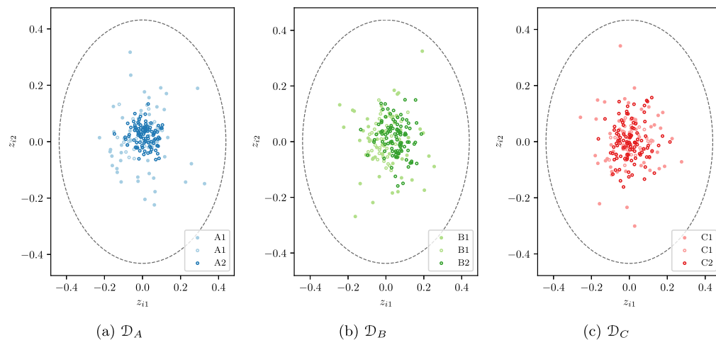
Fig. A13. Domain-wise KPCA. Filled markers \bullet represent training data, hollow markers \circ represent test data. The dashed line shows the 95% confidence ellipse for f .
