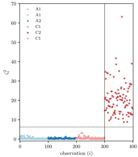
(b) MSD: filled markers \bullet represent training data, hollow markers \circ represent test data. The solid vertical line separates the damage data (C2), the dashed line shows the critical value for damage detection.
