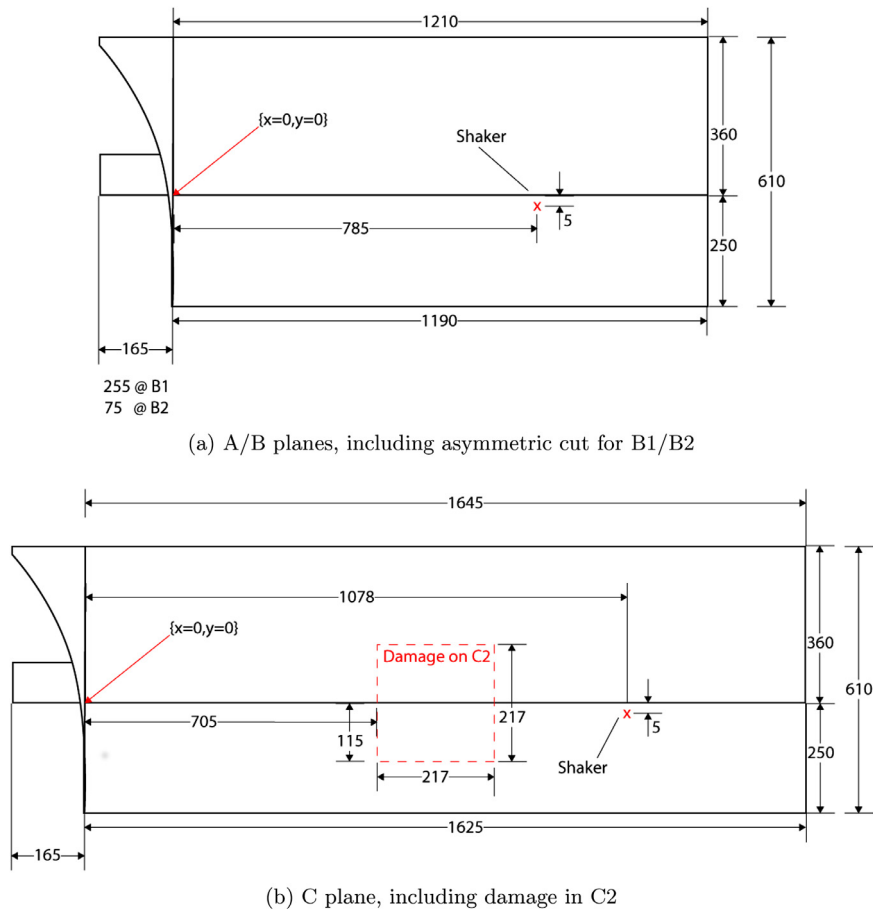
Fig. 2. Schematic, units are in mm. The reference point for scanning is \{x=0, y=0\} . The red cross indicates the forcing location, while the red dashed square shows the artificial damage in C2. (For interpretation of the references to colour in this figure legend, the reader is referred to the web version of this article.)
