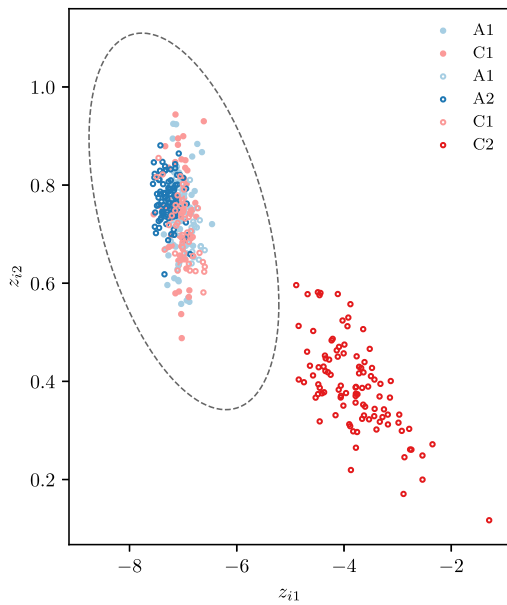
(a) \mathcal{Z} : filled markers \bullet represent training data, hollow markers \circ represent test data. The dashed line shows the confidence ellipse for damage detection.
