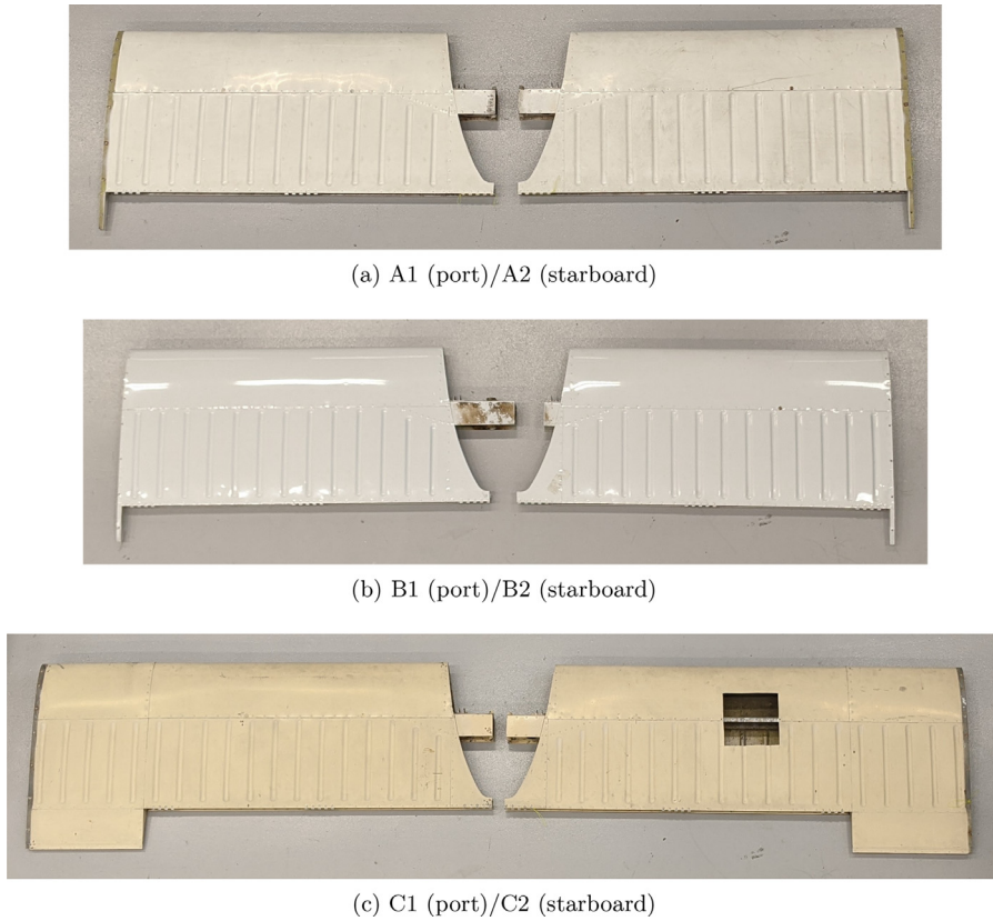
Fig. 3. Tailplane structures, including artificial damage in wing C2 – dimensions are provided in Fig. 2.
