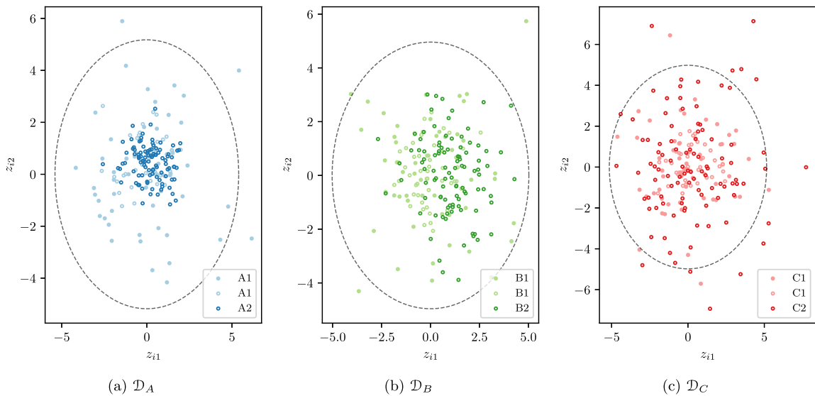
Fig. 8. Domain-wise PCA. Filled markers \bullet represent training data, hollow markers \circ represent test data. The dashed line represents the 95% confidence ellipse for f .
