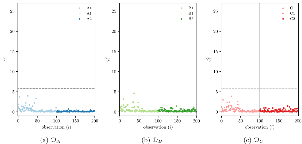
Fig. A14. Domain-wise Mahalanobis distance for KPCA. Filled markers \bullet represent training data, hollow markers \circ represent test data. The solid vertical line separates the damage data (C2), the dashed line shows the critical value for damage detection.
