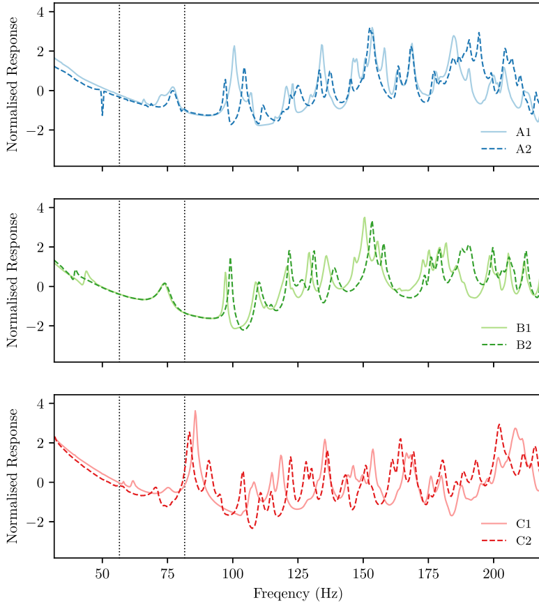
Fig. 6. Frequency response functions for tailplane pairs, normalised in the log-space. Dotted lines highlight the range of consistent features selected for transfer learning.
