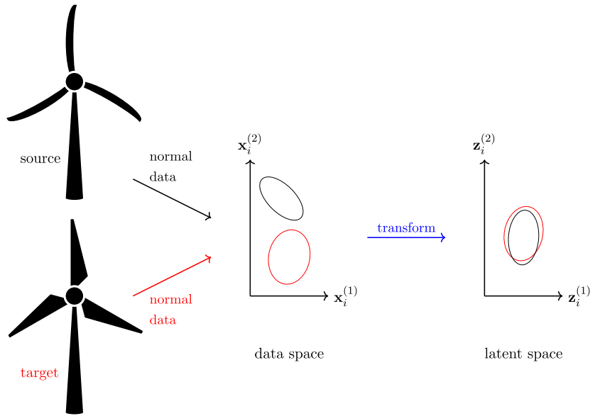
Fig. 1. Visualisation of domain adaptation for knowledge transfer between source and target structures, distribution matching for the normal condition data. Ellipses represent clusters of data from the source (black) and target (red) structures. In the original space \mathbf{x}_i \in \mathcal{X} , the distributions for each structure (i.e. domain) are different; in the latent space \mathbf{z}_i \in \mathcal{Z} (a transformation of \mathbf{x}_i ) the distributions have been (approximately) matched. (For interpretation of the references to colour in this figure legend, the reader is referred to the web version of this article.)
