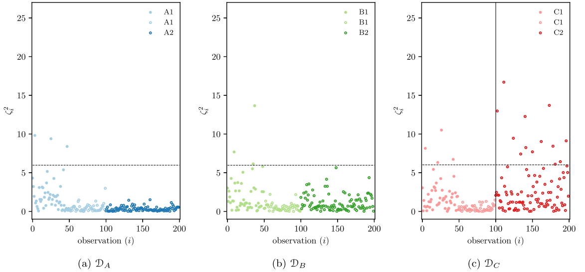
Fig. 9. Domain-wise Mahalanobis distance. Filled markers \bullet represent training data, hollow markers \circ represent test data. The solid vertical line separates the damage data (C2), the dashed line shows the critical value for damage detection.
